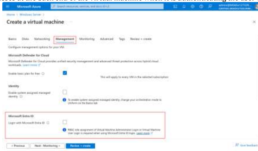
Fig. 5. Step three: VM authenticating user during login
